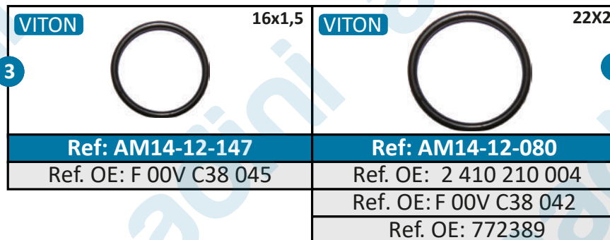
O-ring
